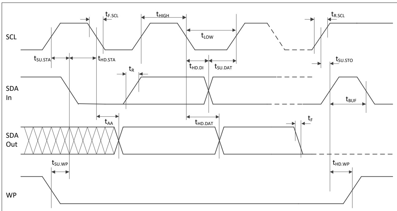
Figure 6–1 Bus Timing
