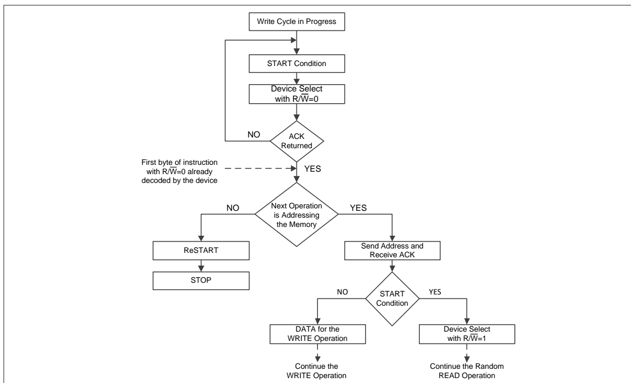
Figure 5-6 Acknowledge Polling Flow Chart
