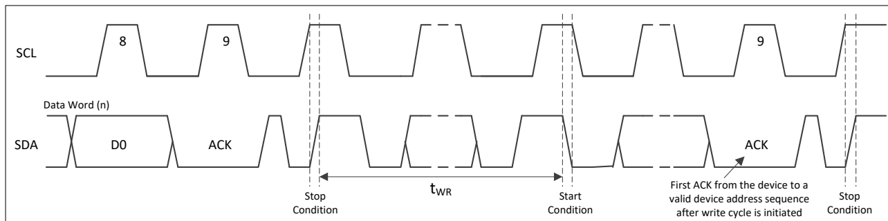
Figure 5-5 Write Cycle Timing
