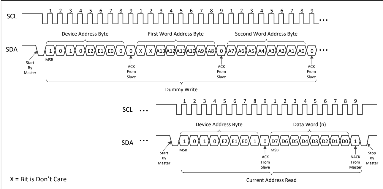
Figure 5-10 Random Read
