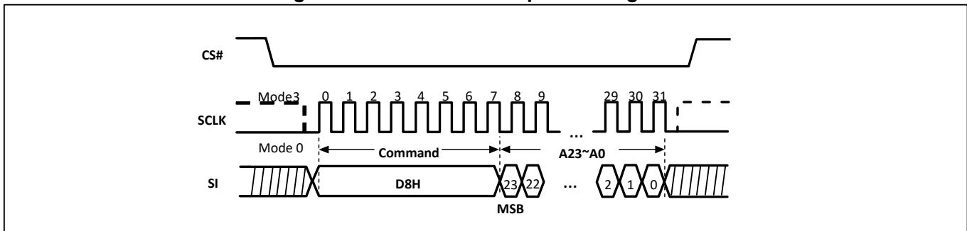
Figure-36. Block Erase Sequence Diagram
