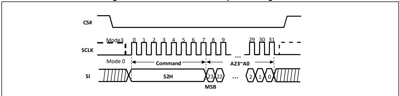
Figure-34. Half Block Erase Sequence Diagram
