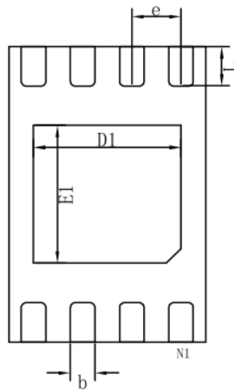
bottom view
