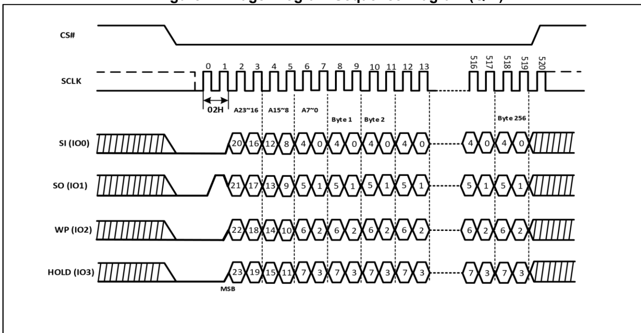
Figure-41. Page Program Sequence Diagram (QPI)
