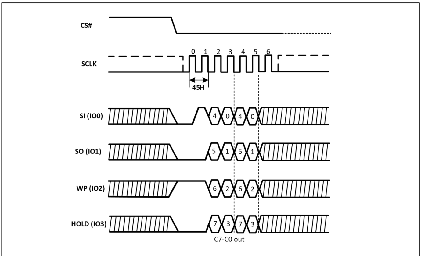
Figure-55. Read Configure Register (QPI)
