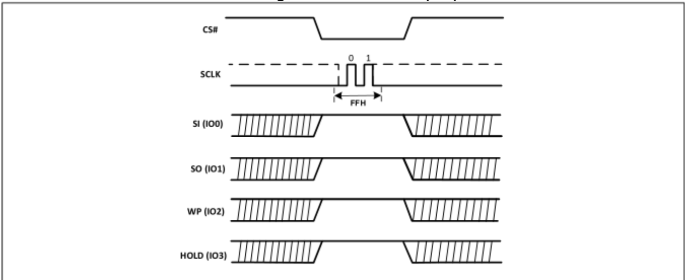
Figure-76. Disable QPI (QPI)
