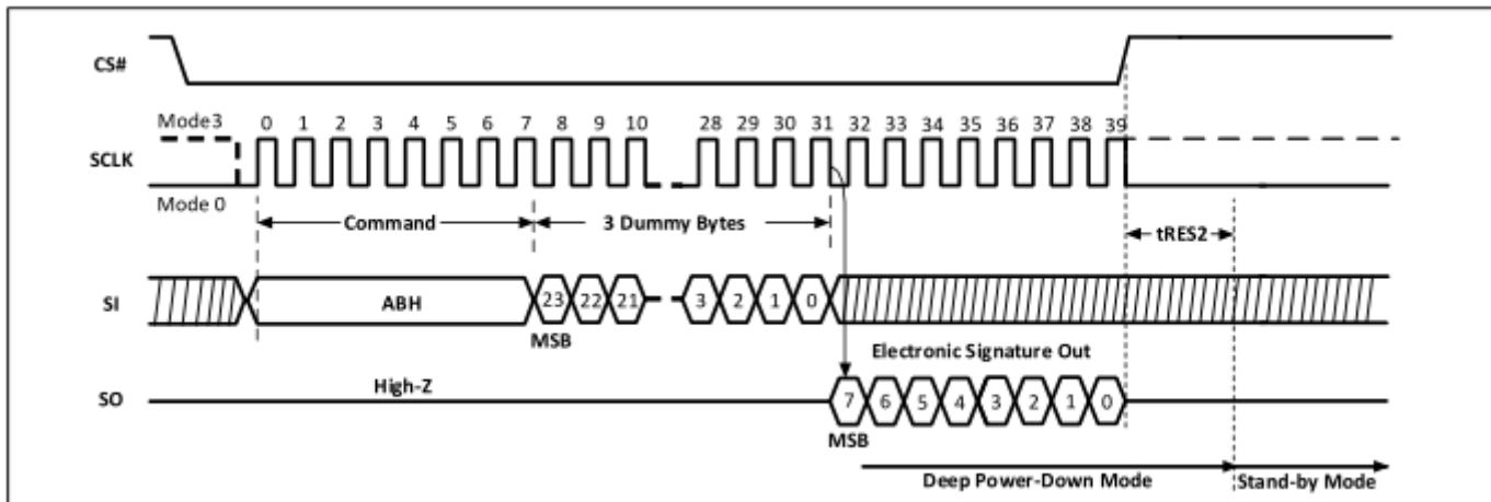
Figure-58. Read Electronic Signature (RES) Sequence Diagram
