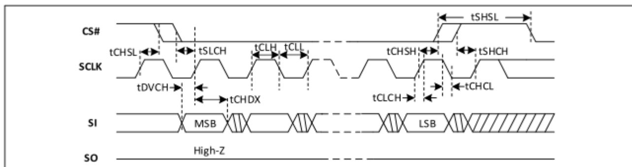
Figure-83. Serial Input Timing
