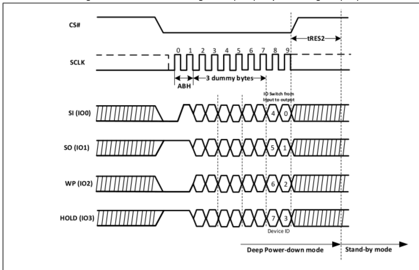
Figure-59. Read Electronic Signature (RES) Sequence Diagram (QPI)
