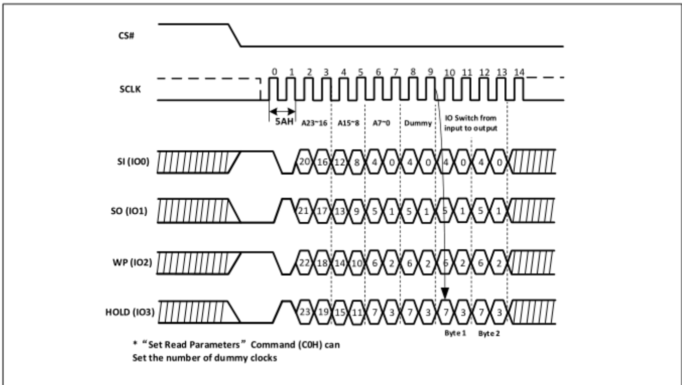
Figure-73. Read Serial Flash Discoverable Parameter Sequence Diagram (QPI)
