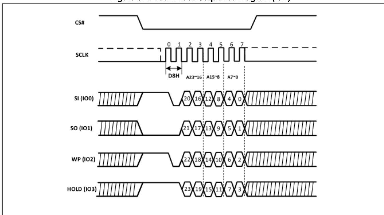
Figure-37. Block Erase Sequence Diagram (QPI)
