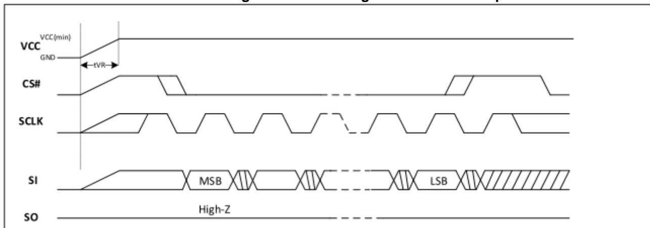
Figure-80. AC Timing at Device Power-Up
