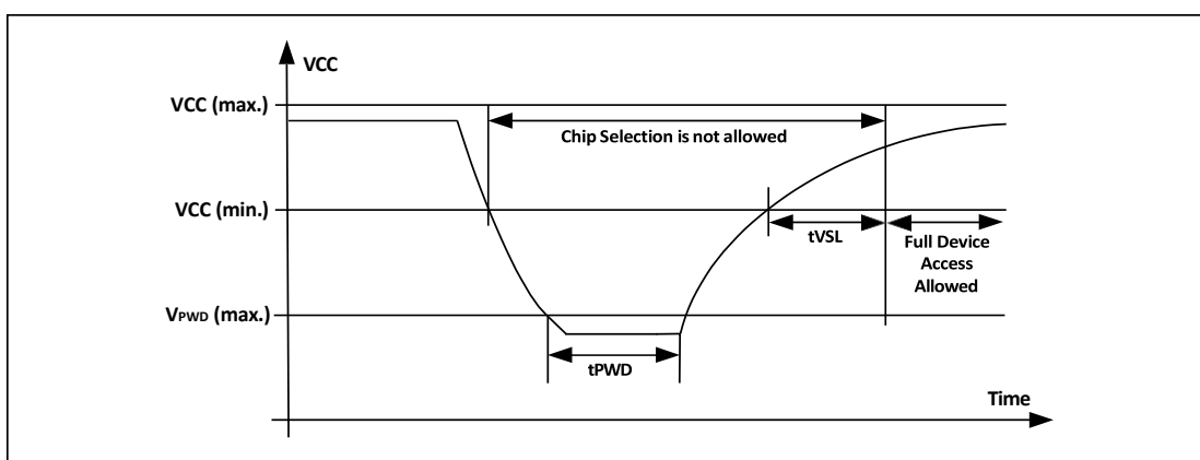
Figure-81. Power-On Timing Sequence Diagram
