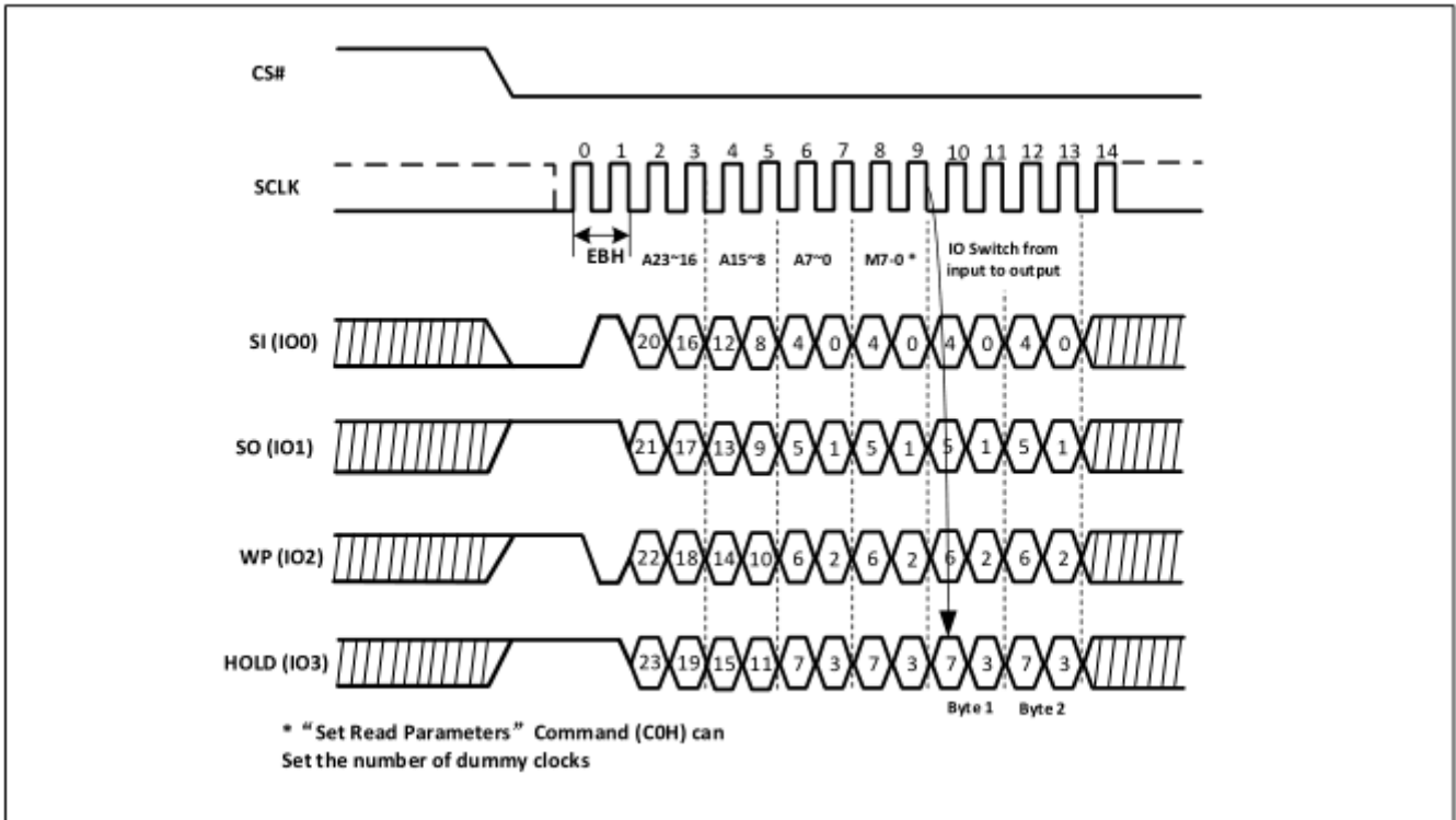
Figure-23. Quad I/O Read in QPI Mode Sequence (M5-4 ≠ (1,0))
