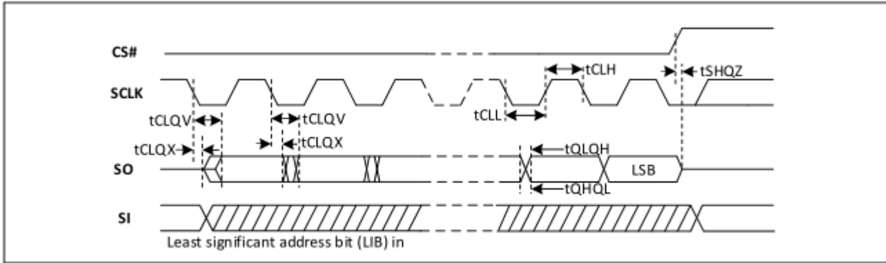
Figure-84. Output Timing
