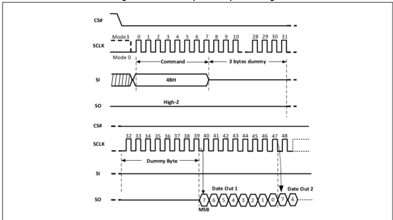
Figure-71. Read Unique ID Sequence Diagram
