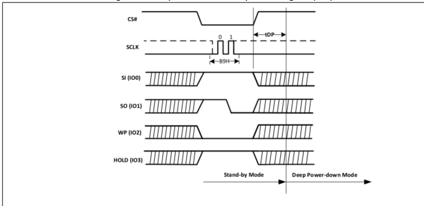
Figure-55. Deep Power-Down Sequence Diagram (QPI)
