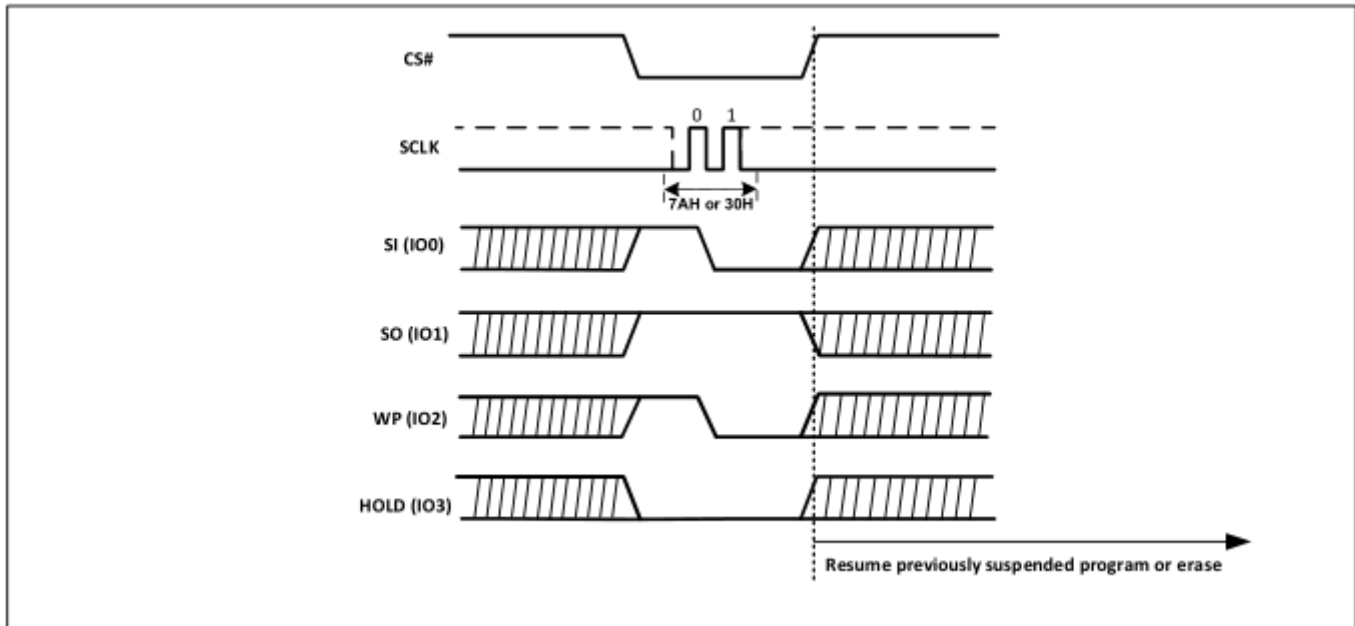
Figure-70. Program Resume and Erase Resume Sequence Diagram (QPI)
