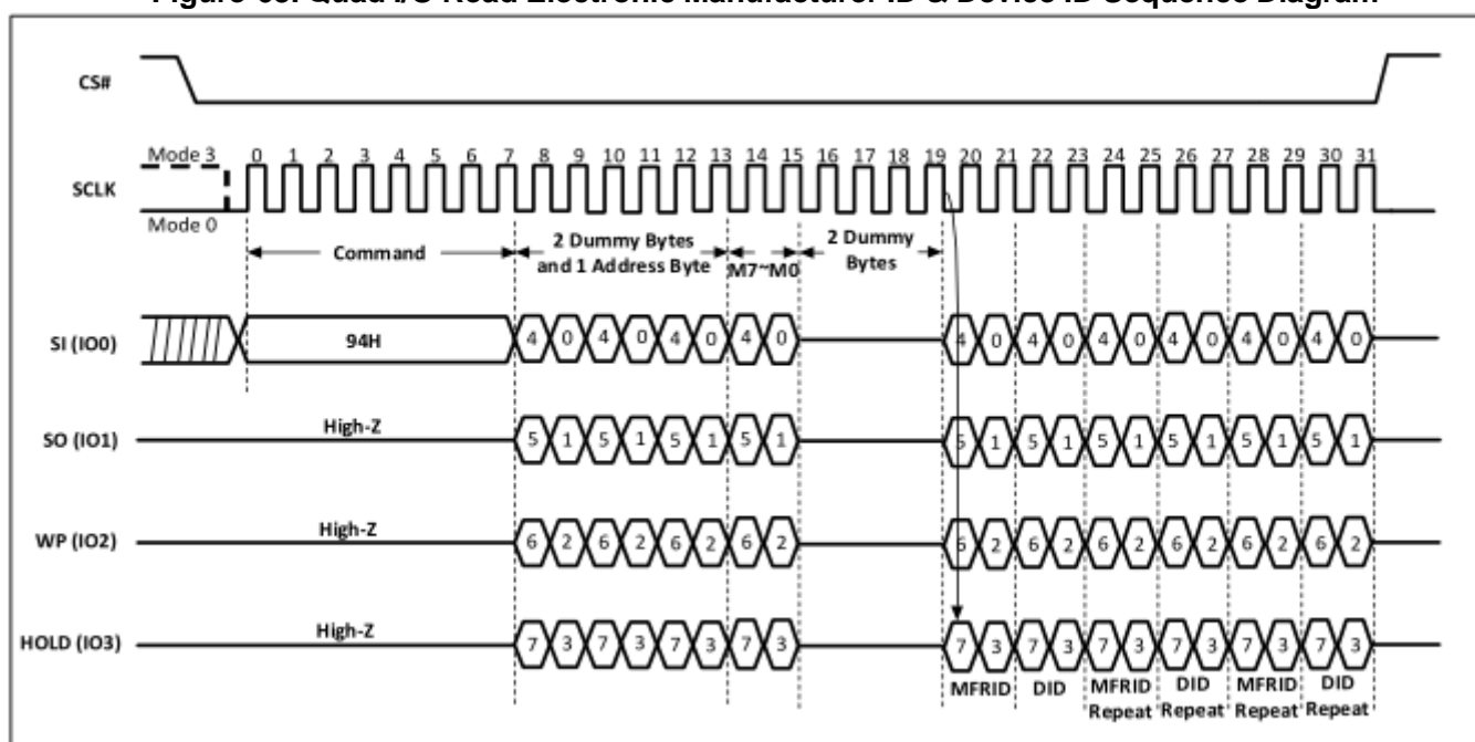
Figure-63. Quad I/O Read Electronic Manufacturer ID & Device ID Sequence Diagram
