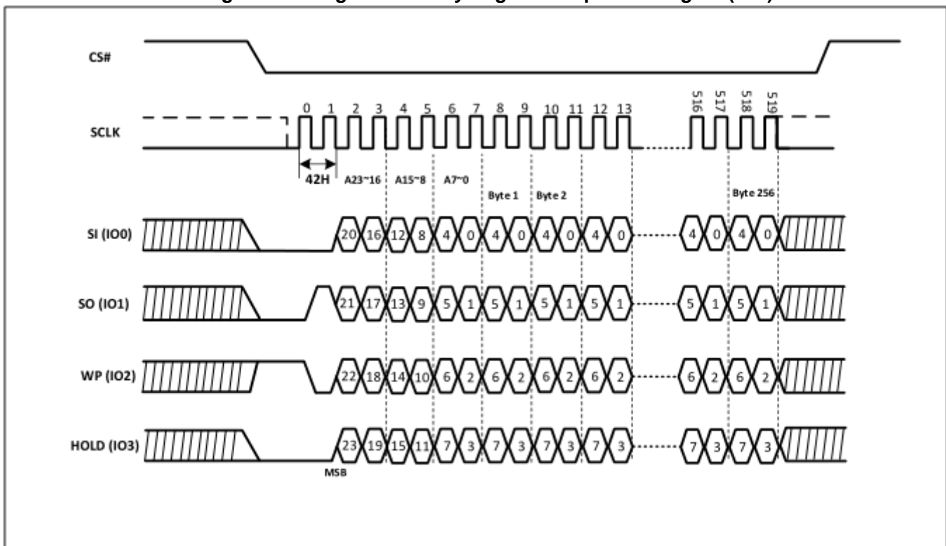
Figure-47. Program Security Register Sequence Diagram(QPI)
