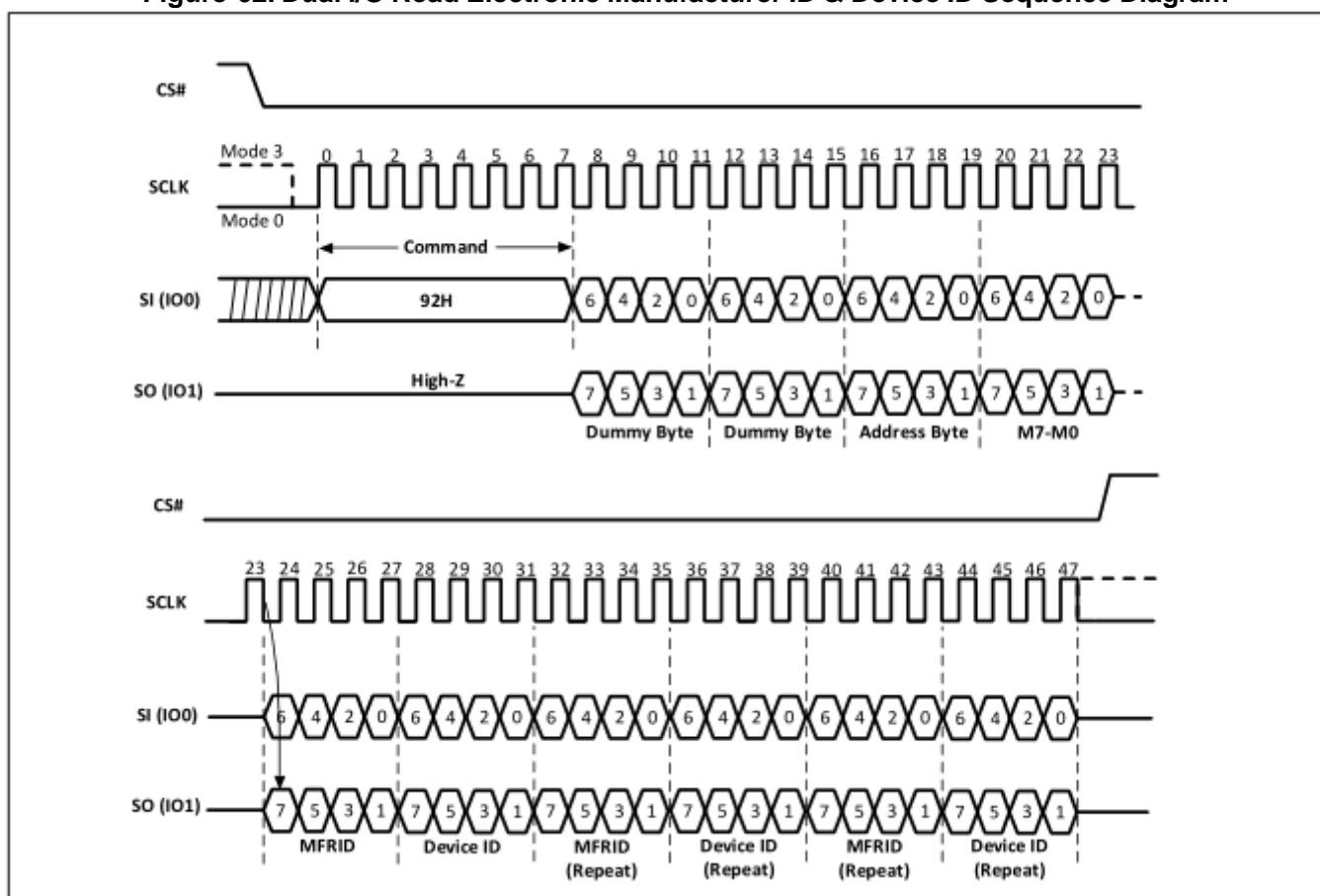
Figure-62. Dual I/O Read Electronic Manufacturer ID & Device ID Sequence Diagram
