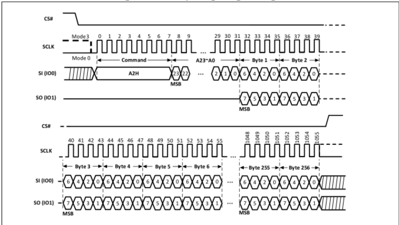
Figure-42. Dual Input Page Program Diagram
