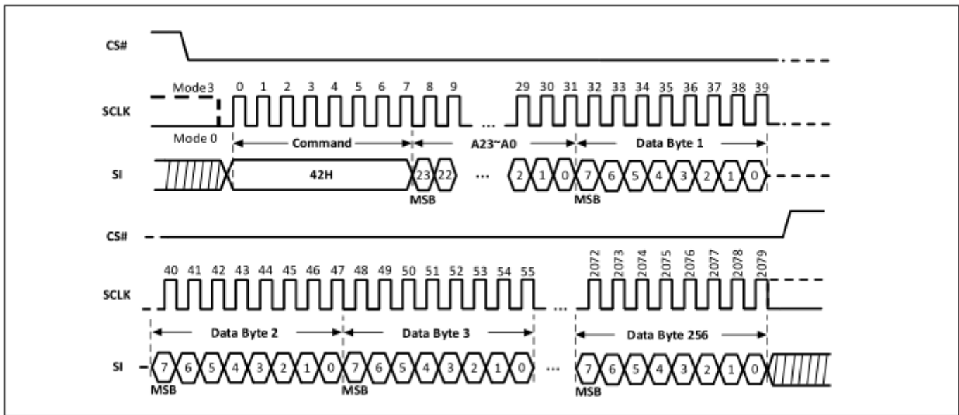
Figure-46. Program Security Register Sequence Diagram
