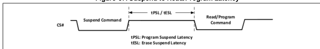
Figure-67. Suspend to Read/Program Latency
