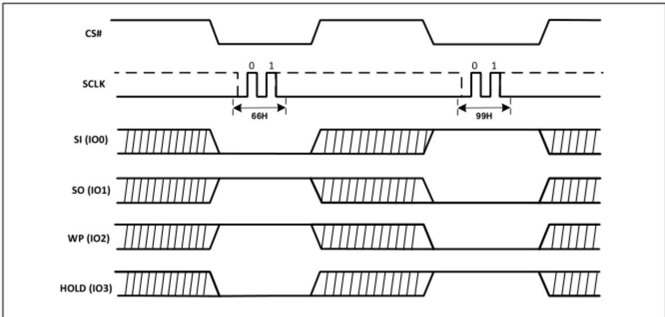
Figure-79 Reset Enable and Reset Sequence Diagram (QPI)
