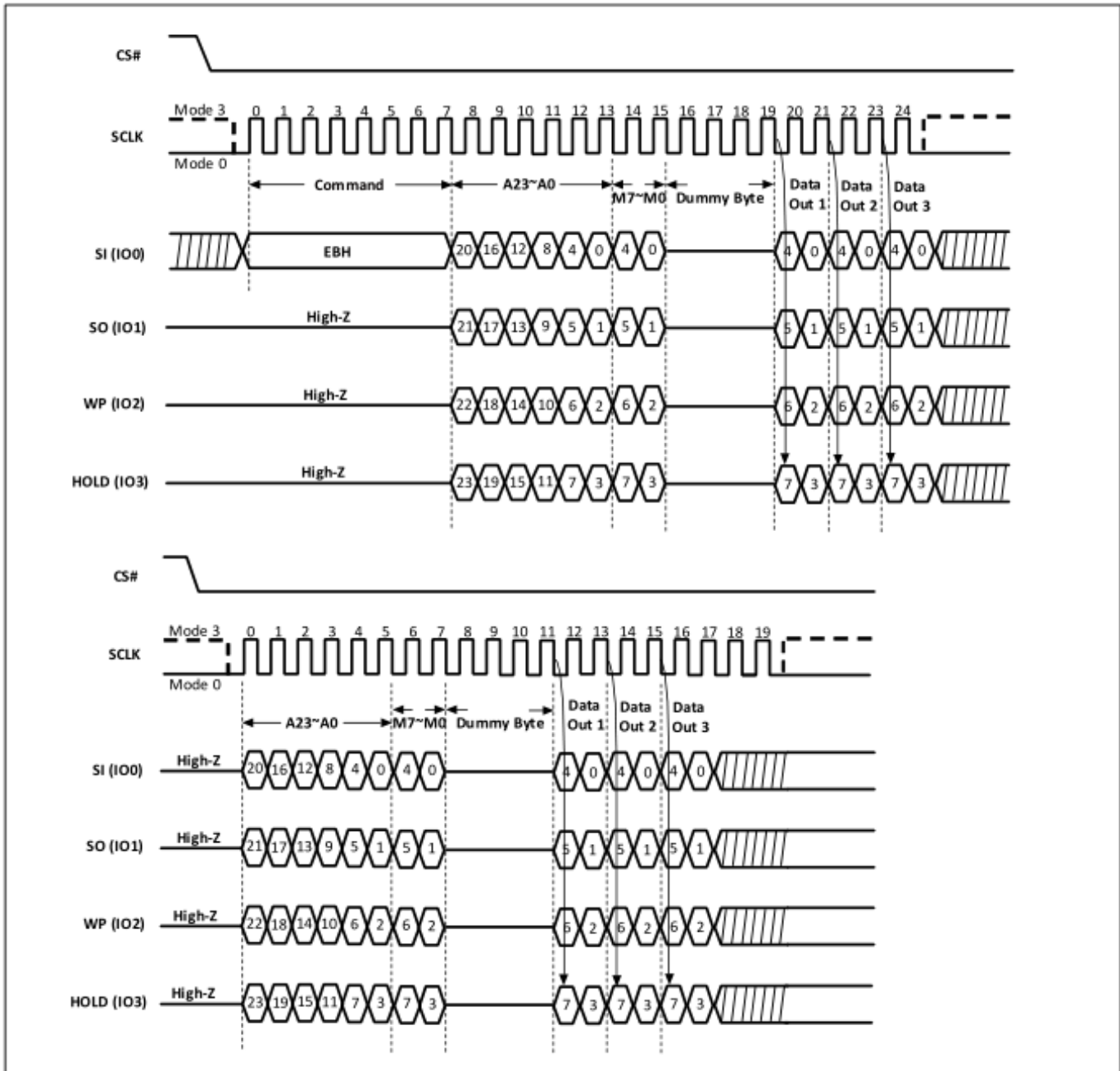
Figure-22. Quad I/O Fast Read with “Continuous Read Mode” Sequence Diagram (M5-4 = (1,0))
