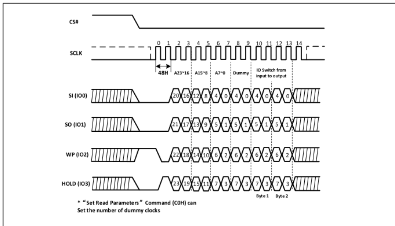
Figure-49. Read Security Register Sequence Diagram (QPI)
