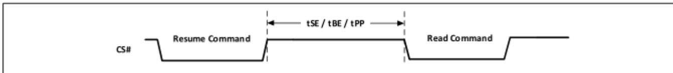
Figure-69. Program Resume and Erase Resume Sequence Diagram
