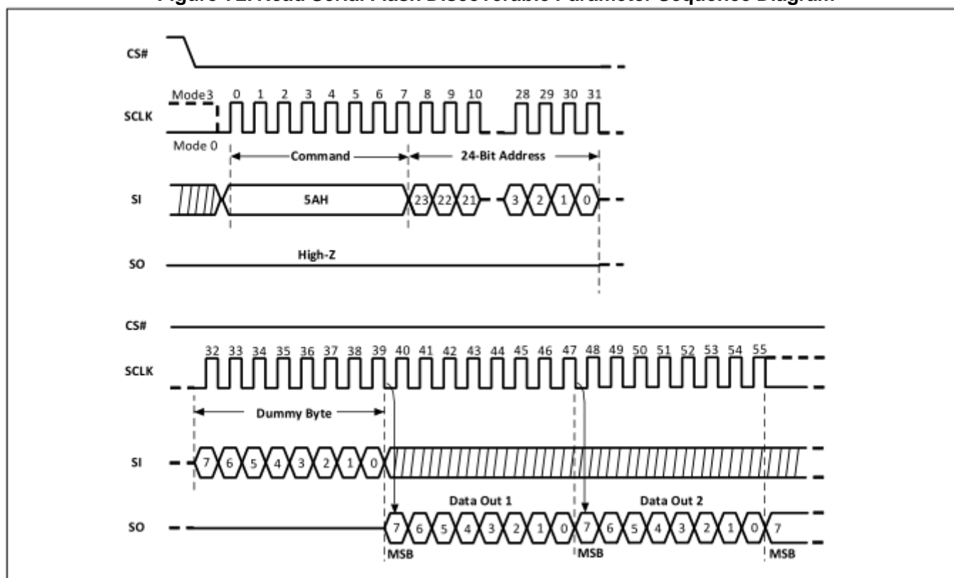
Figure-72. Read Serial Flash Discoverable Parameter Sequence Diagram
