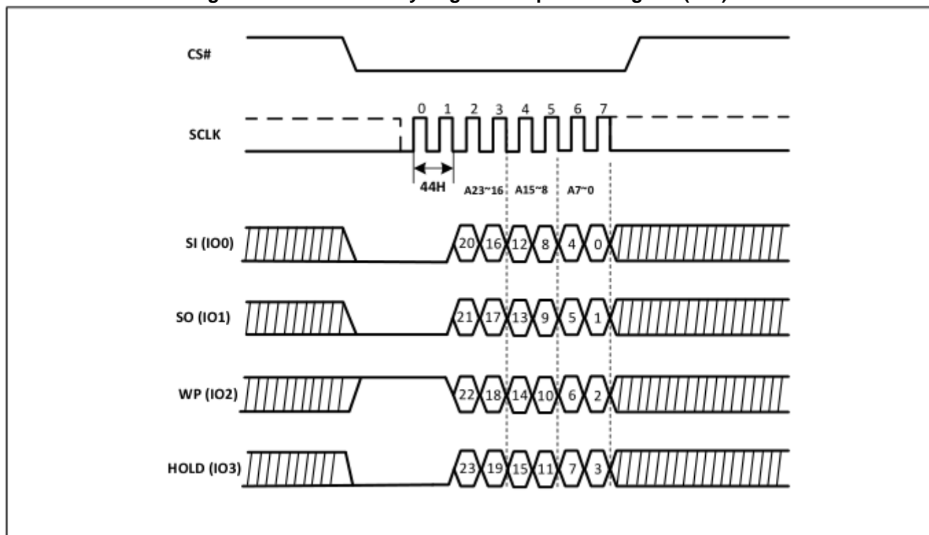
Figure-45. Erase Security Register Sequence Diagram (QPI)
