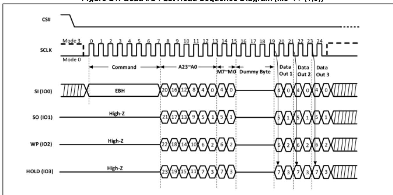
Figure-21. Quad I/O Fast Read Sequence Diagram (M5-4 ≠ (1,0))
