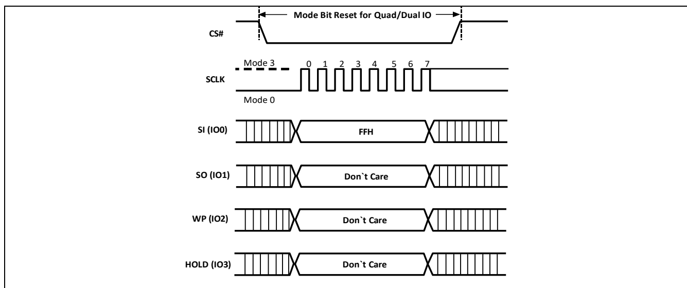
Figure-74. Continuous Read Mode Reset Sequence Diagram
