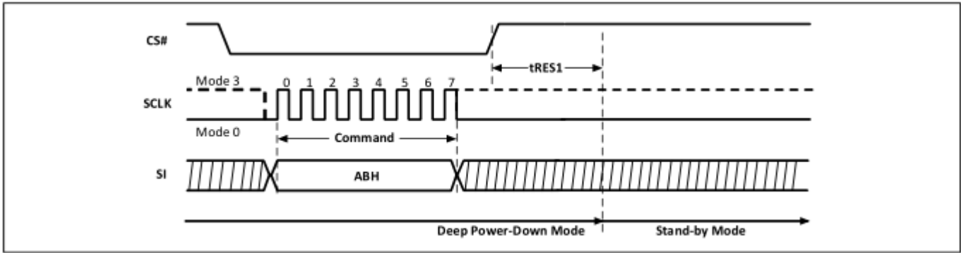
Figure-57. Release from Deep Power-Down (RDP) Sequence Diagram (QPI)
