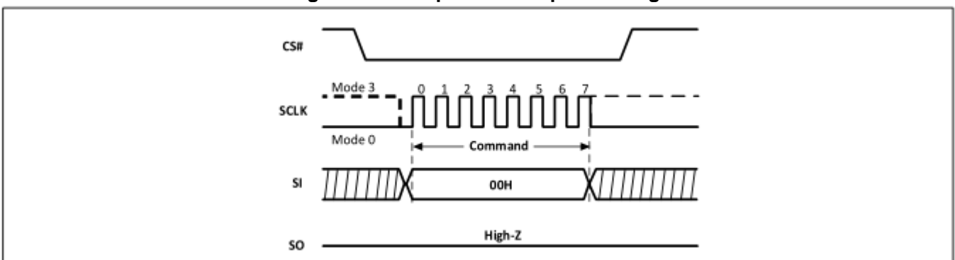
Figure-77. No Operation Sequence Diagram
