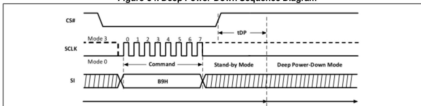
Figure-54. Deep Power-Down Sequence Diagram
