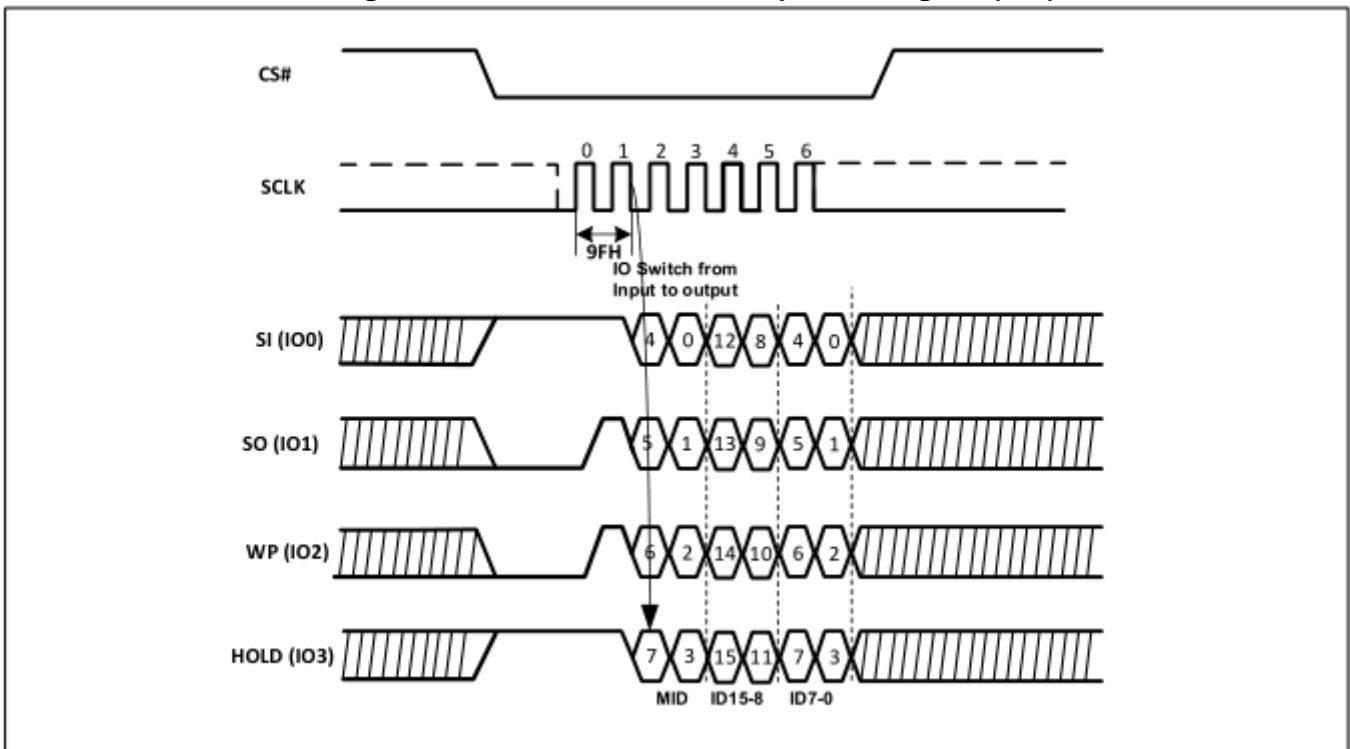
Figure-65. Read Identification Sequence Diagram (QPI)
