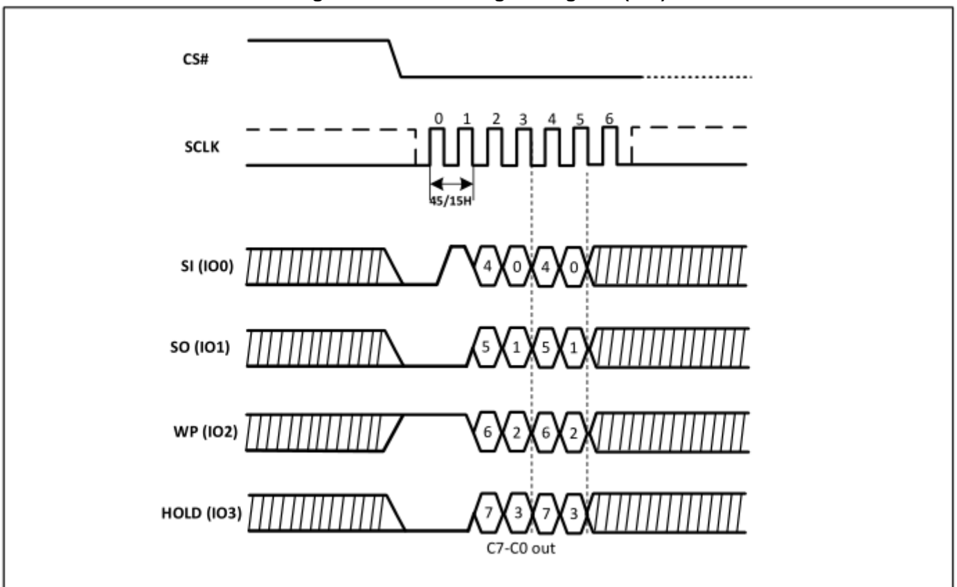
Figure-53. Read Configure Register (QPI)
