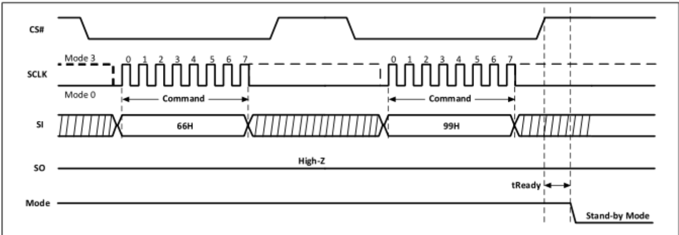
Figure-78. Reset Enable and Reset Sequence Diagram
