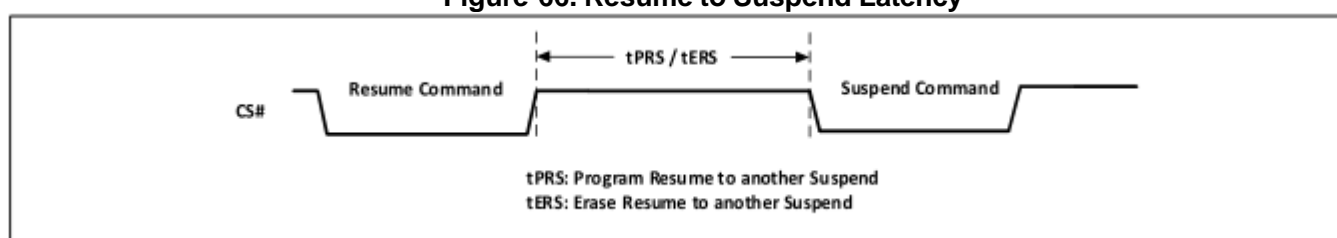
Figure-66. Resume to Suspend Latency
