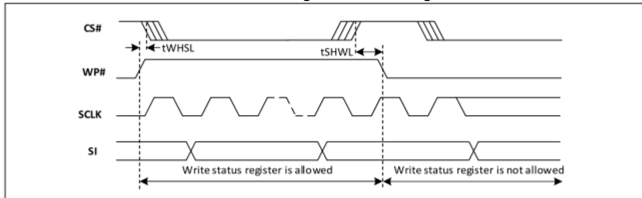
Figure-86. WP Timing
