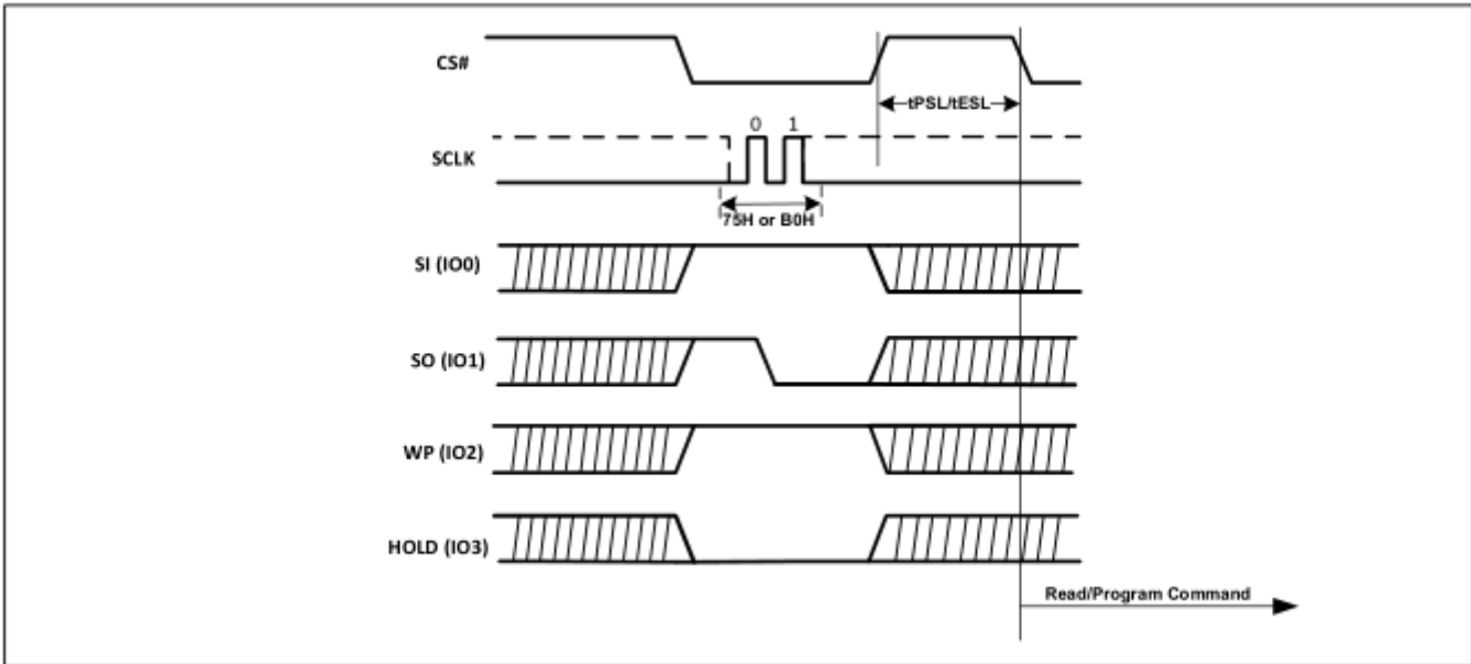
Figure-68. Suspend to Read/Program Latency (QPI)
