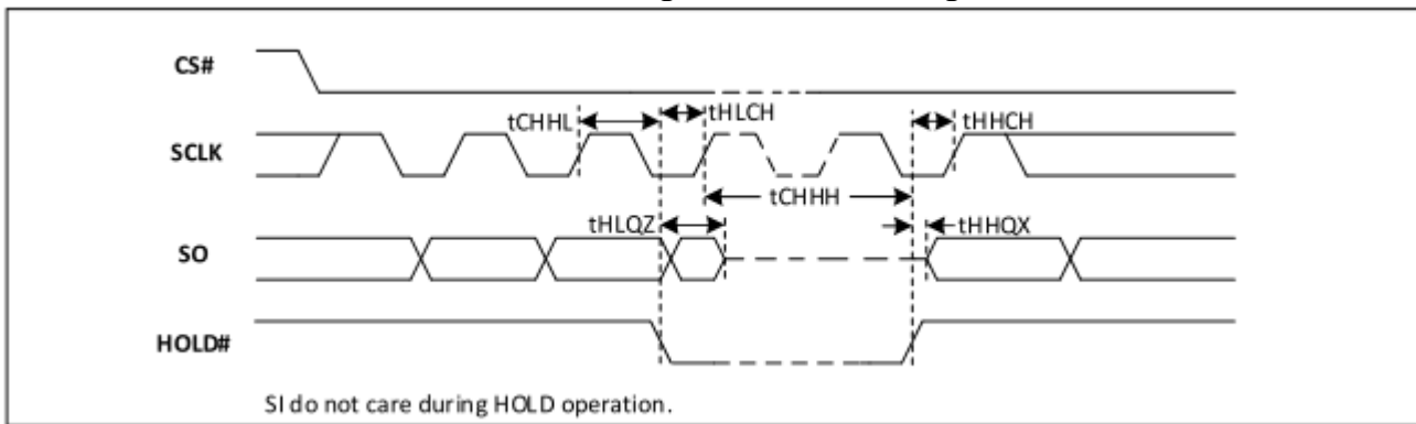
Figure-85. Hold Timing
