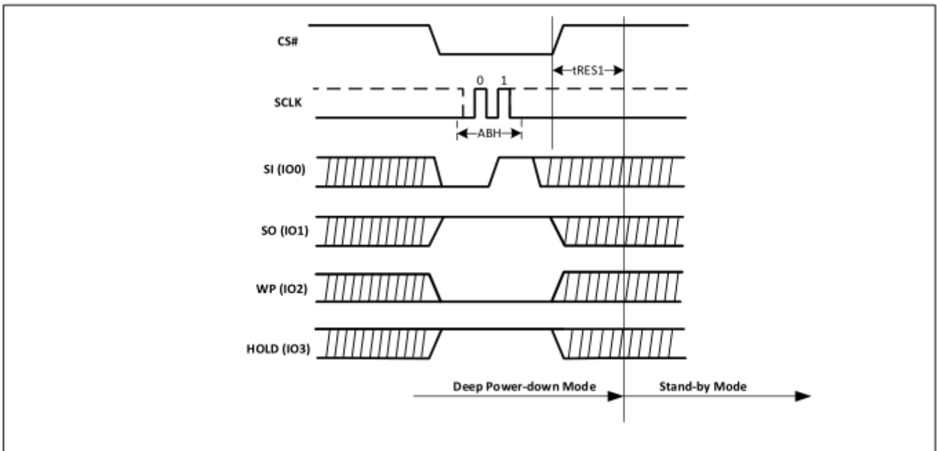
Figure-58. Read Electronic Signature (RES) Sequence Diagram
