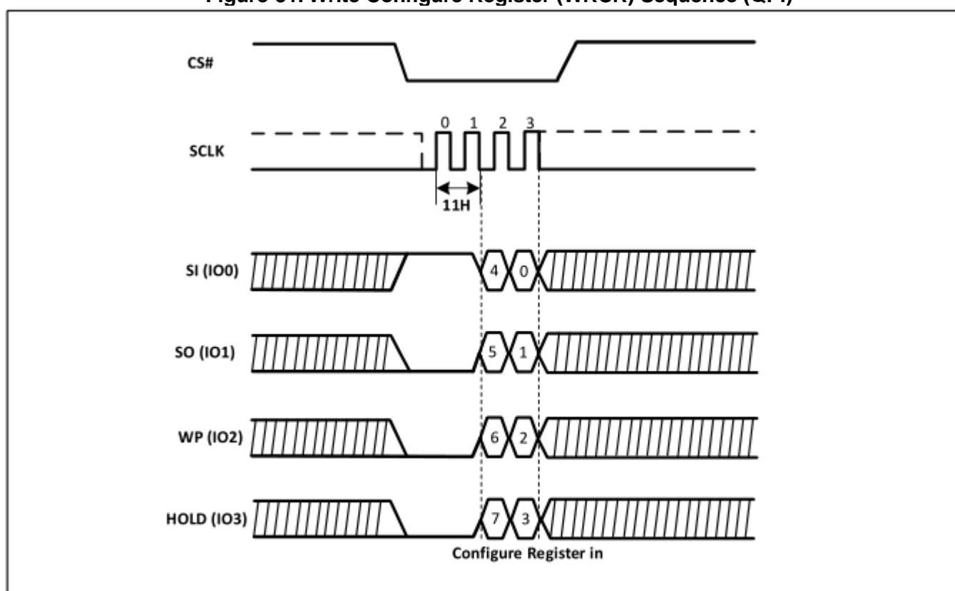
Figure-51. Write Configure Register (WRCR) Sequence (QPI)
